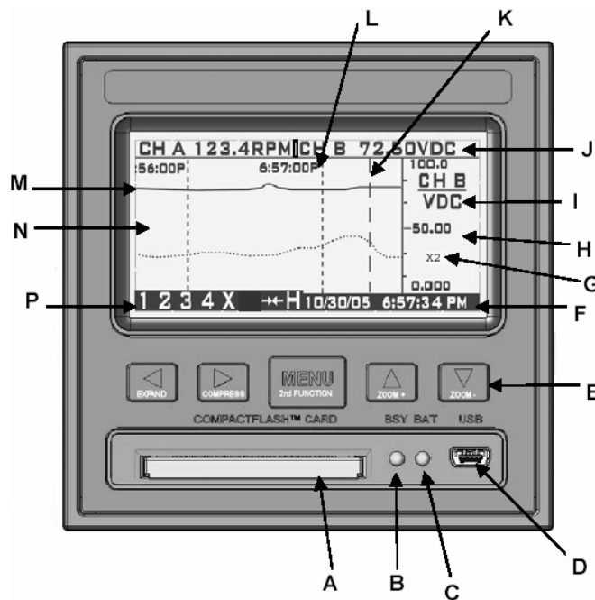
Recorder Front View showing TREND Display
