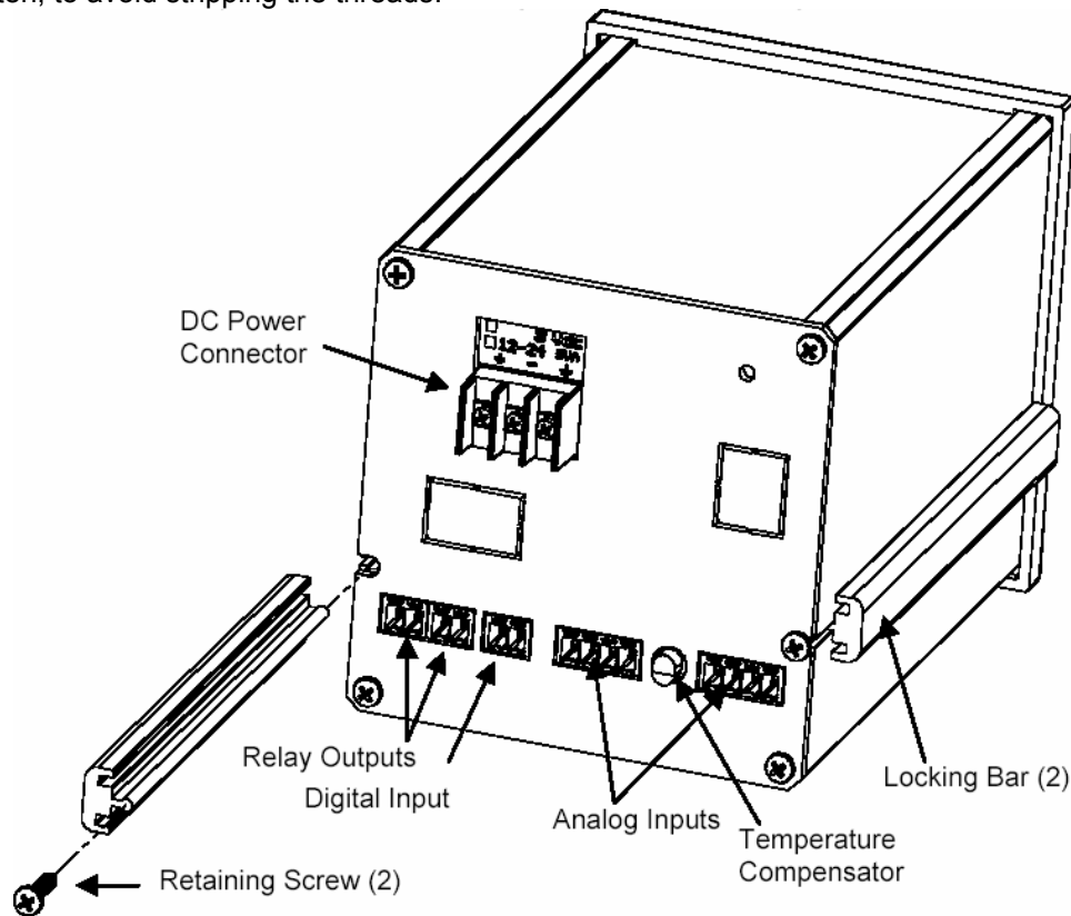
Figure 2.2 Rear View - Installation
