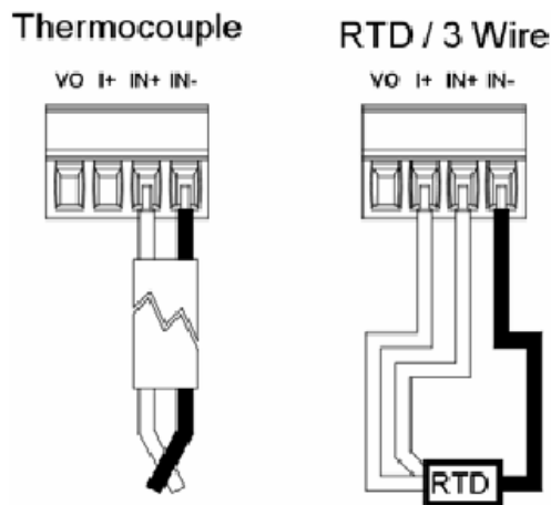
Figure 2.4 - Connection Detail
